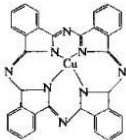
Chemical Structure
